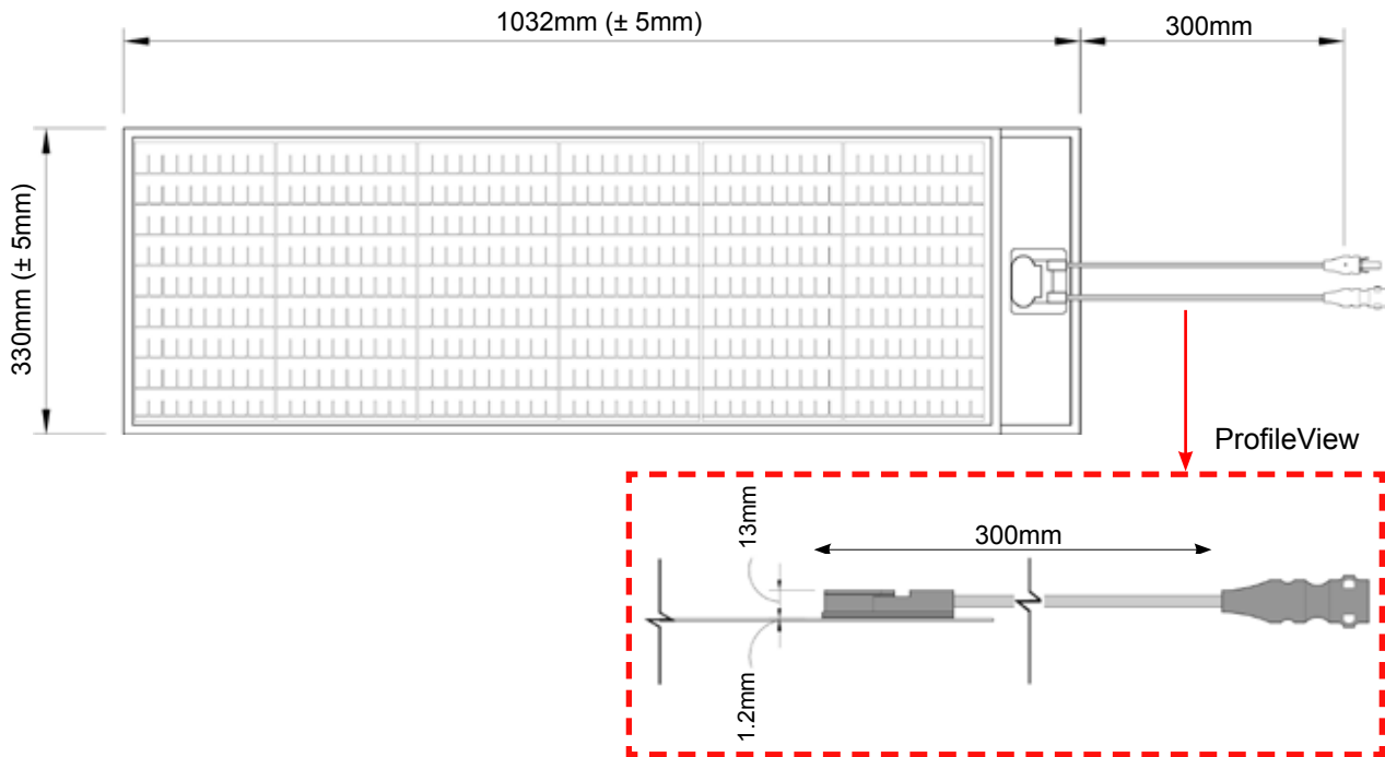
WaveSol Light 1-Meter Back Side View
