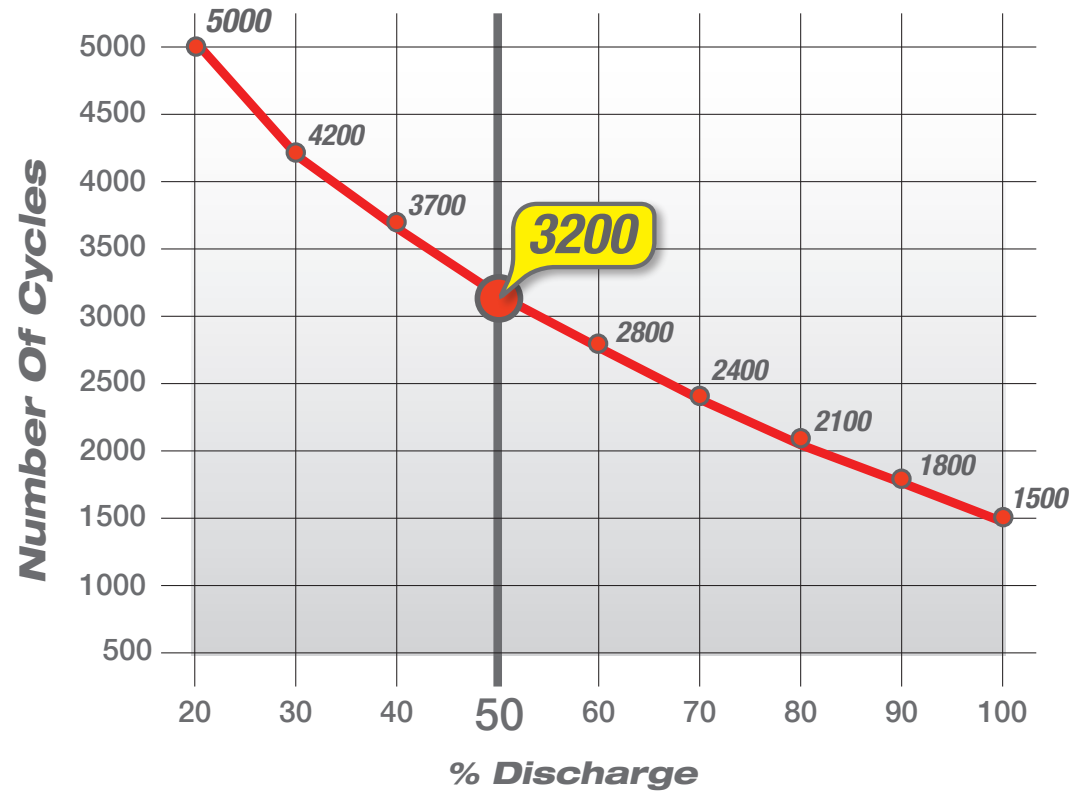
Cycle Life vs. Depth of Discharge
